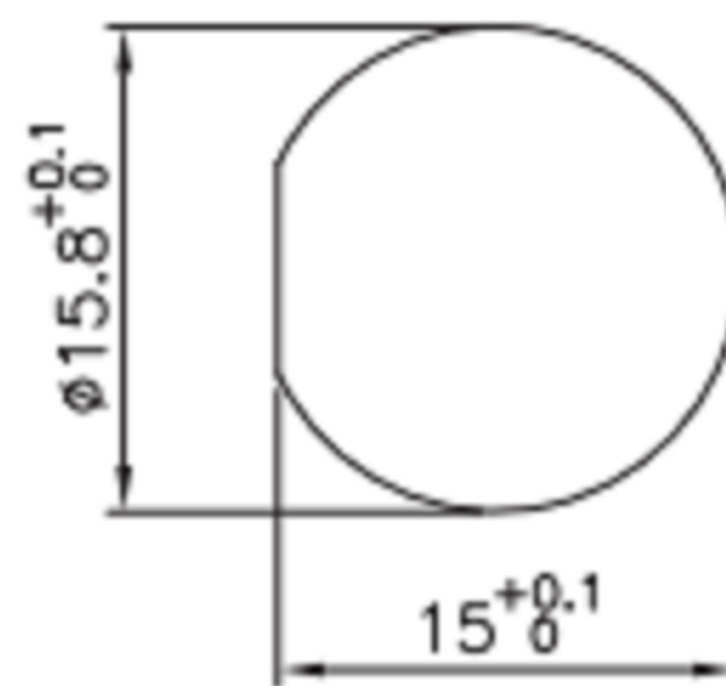
开孔尺寸 hole opening size
